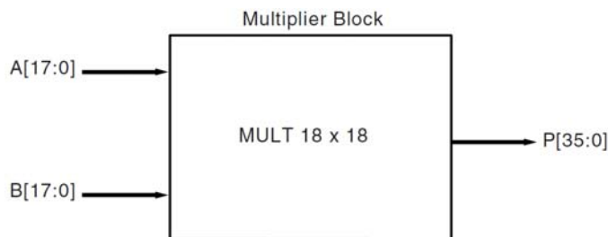
Figure 29 Multiplier Block
