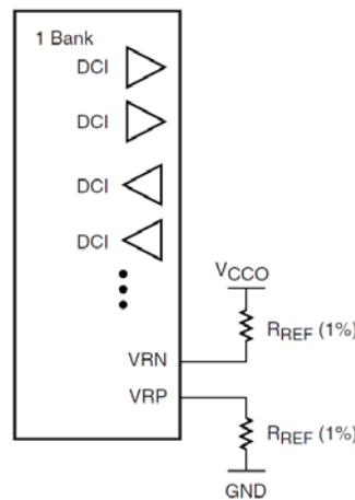
Figure 7 DCI in a BQR2V3000 Bank
