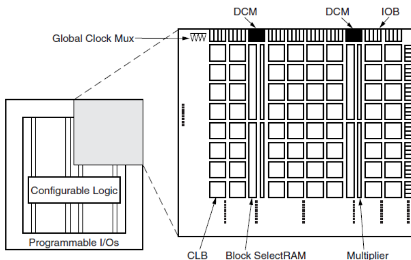
Figure 1 BQR2V3000 Architecture Overview
