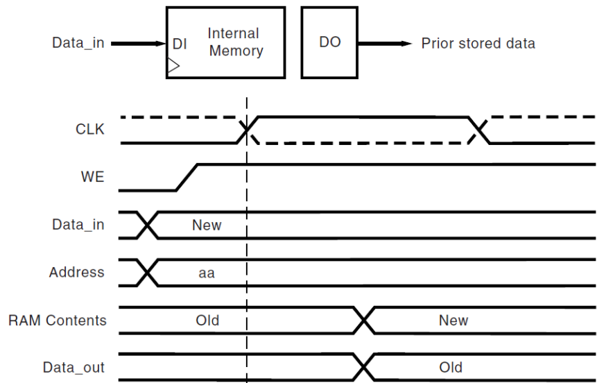
Figure 25 READ_FIRST Mode
