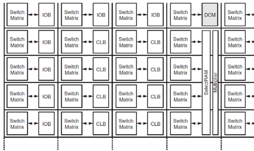
Figure 41 Routing Resource
