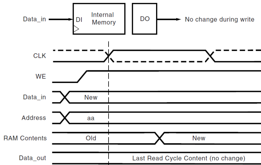
Figure 26 NO_CHANGE Mode
