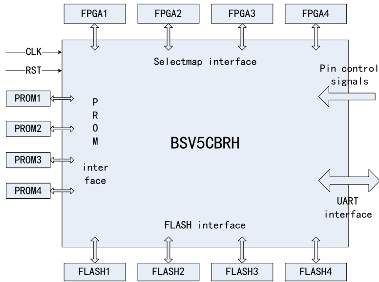
Figure 4-1 BSV5CBRH function block diagram
